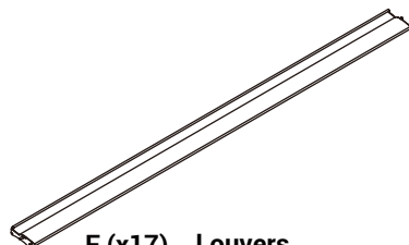
F (x17) Louvers 9'-5 3/8" x 1 5/16" (2879*195*33.2mm)
